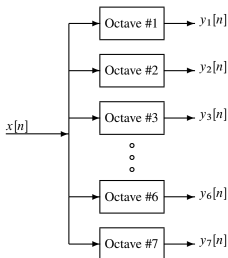
Figure 3: Filter bank consisting of bandpass filters which pass frequencies corresponding to the seven octaves on a piano. (Each octave contains 12 keys, but we will ignore the four extra keys outside the seven complete octaves.)
