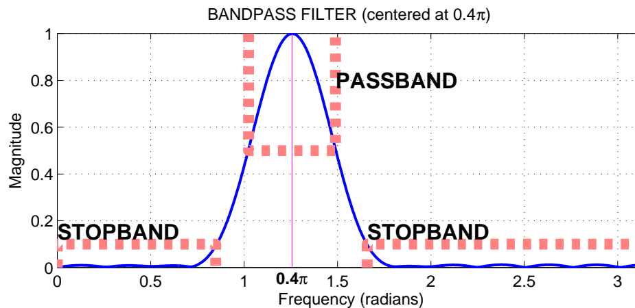
Figure 2: The frequency response of an FIR bandpass is shown with its passband and stopband regions. In this case, the passband is defined to be the region where |H(e^{j\hat{\omega}})| is greater than 0.5; and the stopband is the region where the magnitude is less than 0.1.
